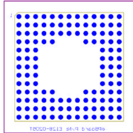
Mill-Max PGA Socket (510-93-132-13-041001)
