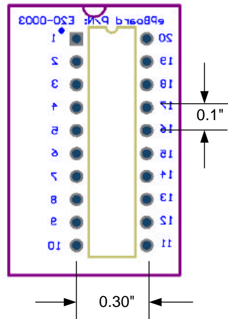
Bottom Side (Top View X-Ray)
