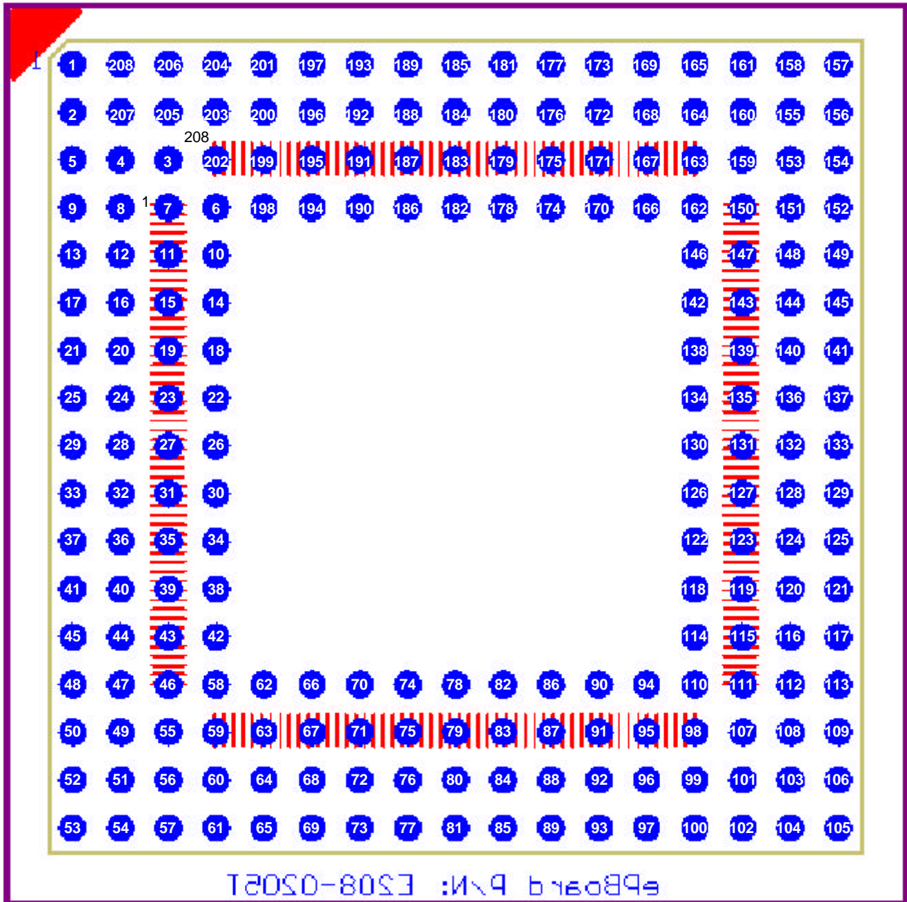
Top View X-Ray with PGA pin assignment
