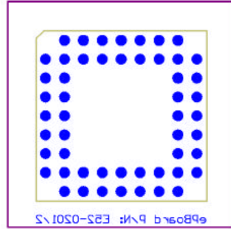
Mill-Max PGA (9x9)Socket (510-93-052-09-045001)
