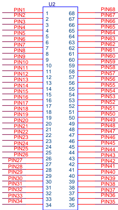
PGA68 11x11
