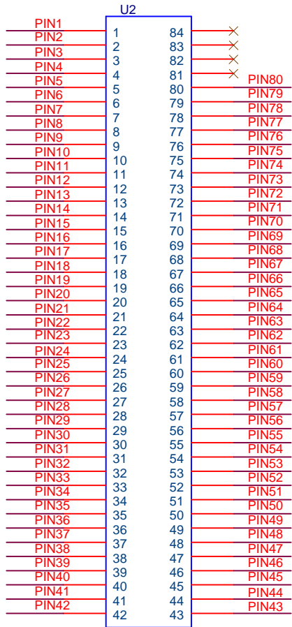
PGA84 (10x10x3)
