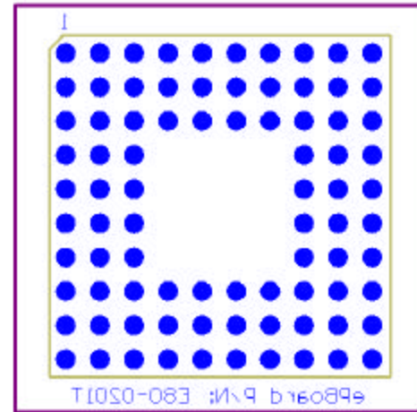
Mill-Max PGA Socket (510-93-084-10-031)
