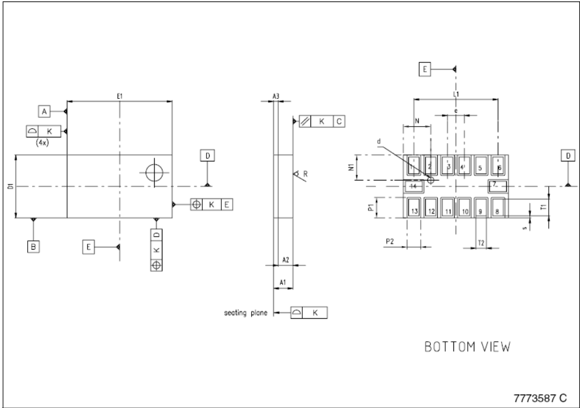
LGA14 (3x5x0.92mm) Pitch 0.8mm Land Grid Array Package
